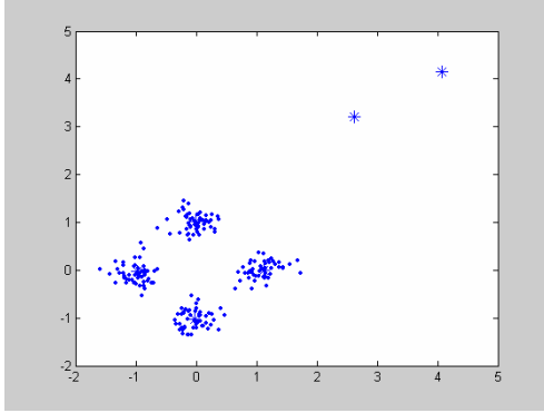
Fig. 6: The clustering result using an improved RPCL algorithm when k is set to 6. Note that there are 2 ( k-4 ) redundant neurons that have been isolated from the cluster area and at the same time there is no cluster center that has deviated from the mean.
