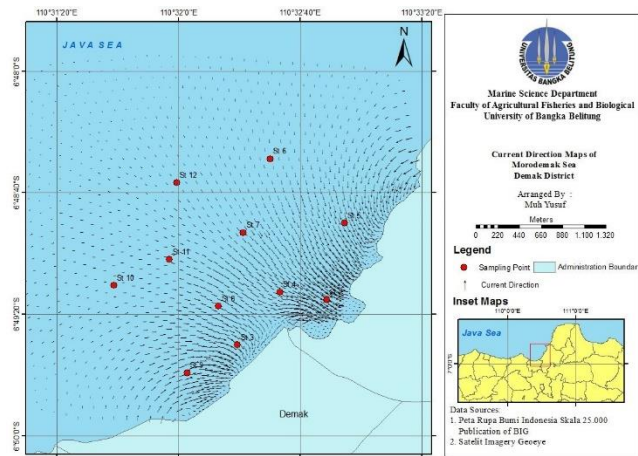
Fig. 3. Spatial surface current profile at Morodemak-Demak
