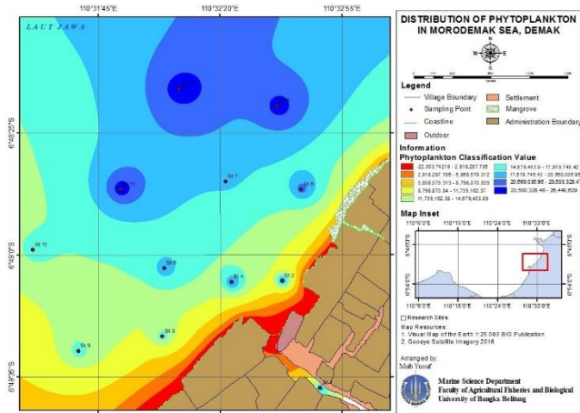
Fig. 2. Spatial distribution of phytoplankton at Morodemak-Demak
