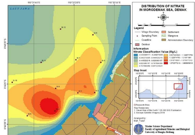
Fig. 1. Spatial distribution of nitrate at Morodemak-Demak
