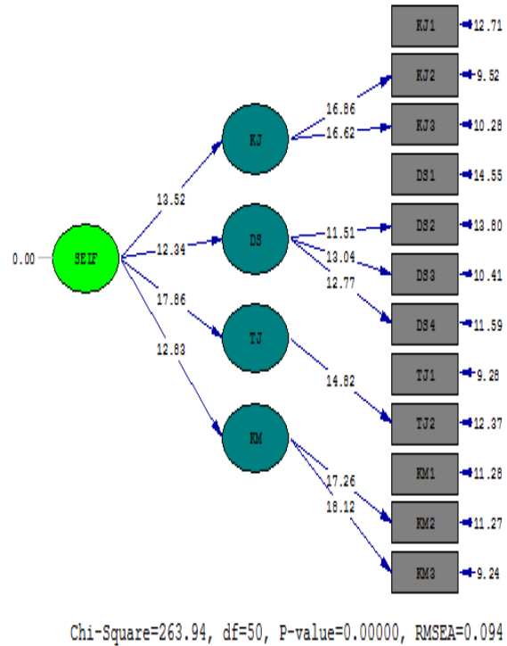
Fig. 1. CFA second-order diagram based on standardized solution
