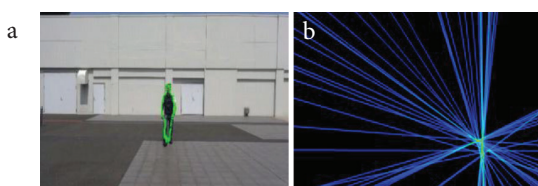
Figure 1 | Extension of optical flow lines: (a) Optical flow detected from a human motion, (b) FoE on a voting plane.
