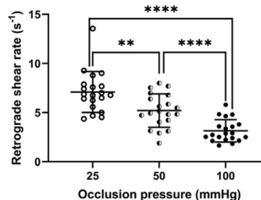
Rise in retrograde shear rates at different grades of supra-systolic occlusion pressures
