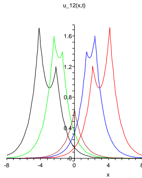
Fig. 2. The two-peakon dynamic for the potential u_{12}(x, t) in (4.7). Red line: t = -2 ; Blue line: t = -1 ; Brown line: t = 0 (collision); Green line: t = 1 ; Black line: t = 2 .
