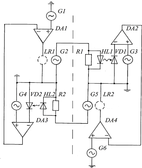
Fig 2. Key diagram of reciprocity
