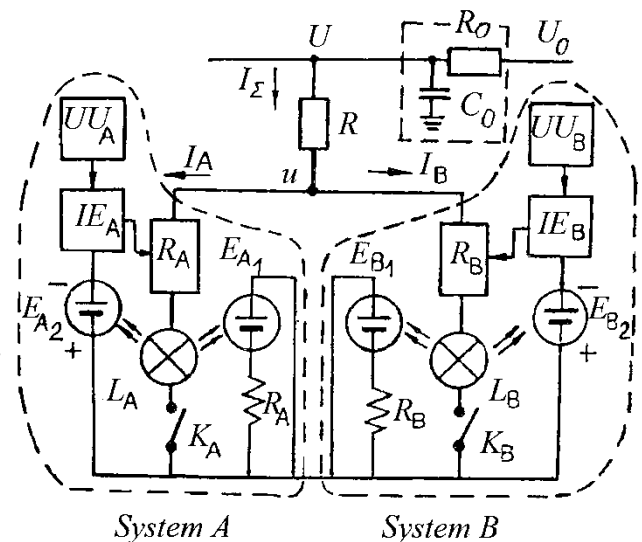
Fig. 1. Electric circuit of system interaction
