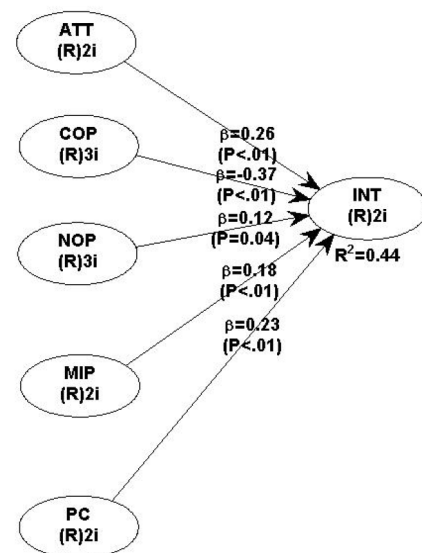
Figure 2 | Inner model test results. Source: Research results (2019).
