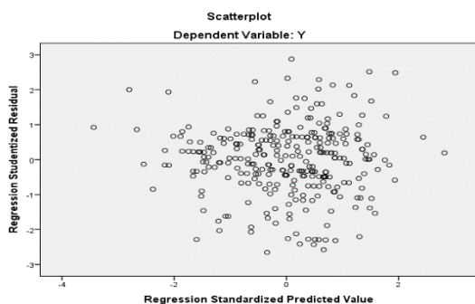
Fig. 2. Scatterplot of heteroscedasticity test.
