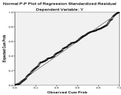
Fig. 1. Scatterplot normality test.
