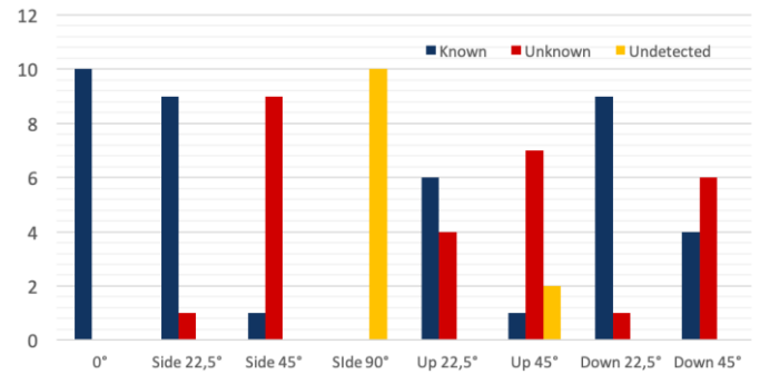
Fig. 3. Face recognition accuracy.
