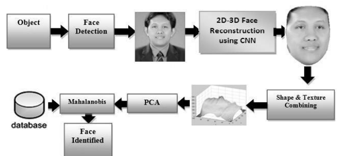
Fig. 1. Face presence system using hybrid method.
