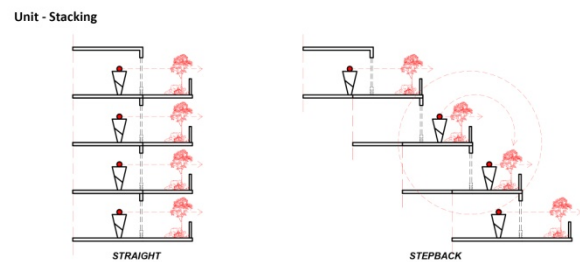
Figure 15 Unit - Stacking
