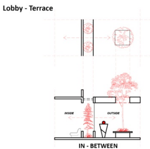
Figure 13 Lobby - Terrace
