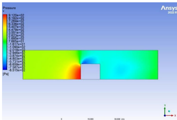
Figure 6: the pressure distribution of flat-roofed house
