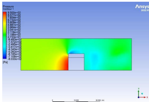
Figure 5: the pressure distribution of gable-roofed house
