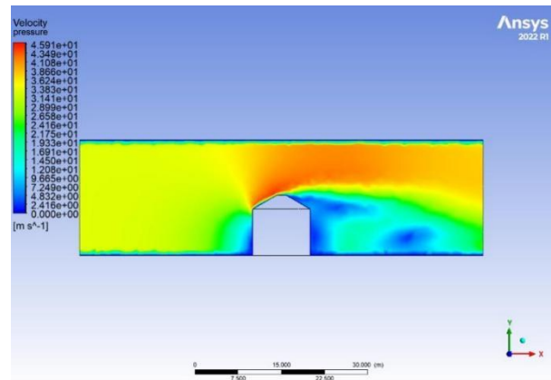
Figure 1: the velocity distribution of hip-roofed house
