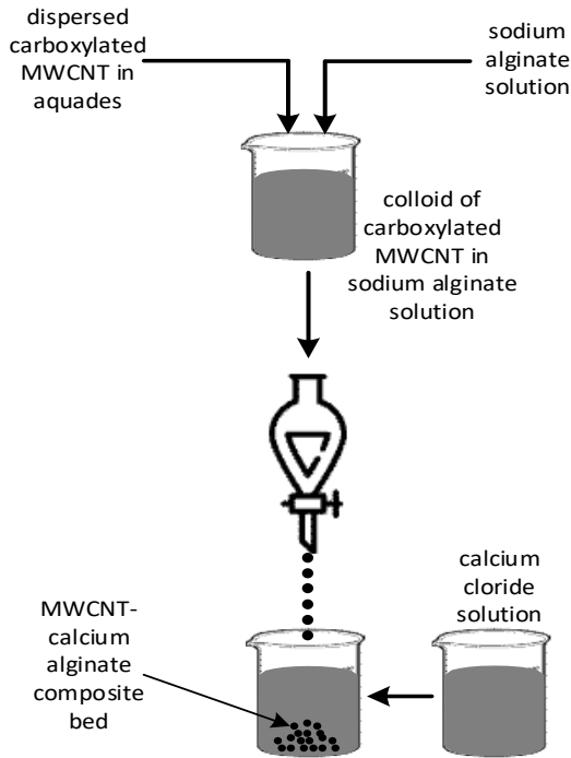
Fig. 1. Illustration of the process of synthesis of a composite of PWNC/ calcium alginate using the impregnation method.
