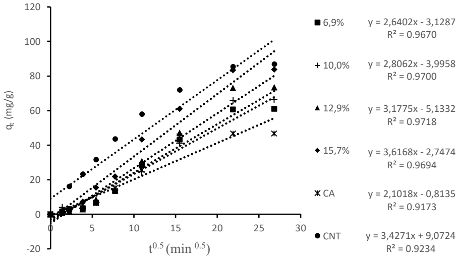
Fig. 4. Plot of the kinetic model of diffusion in a pore.
