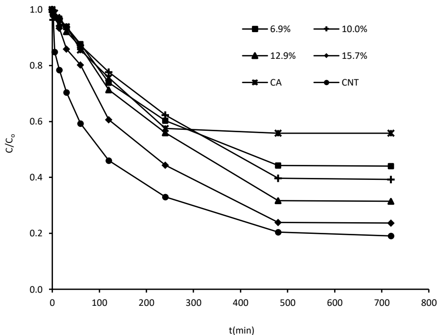
Fig. 3. Adsorption profile of MB on PWNC/calcium alginate composite with variations in carbon nanotube dosage.
