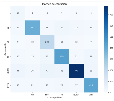
Fig. 2. Confusion Matrix for CNN
