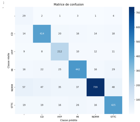
Fig. 8. Confusion Matrix for LSTM
