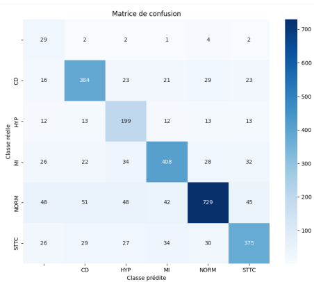
Fig. 6. Confusion Matrix for U-net
