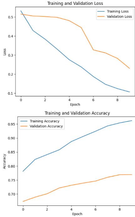
Fig. 7. Training and Validation Loss/ Accuracy for U-net
