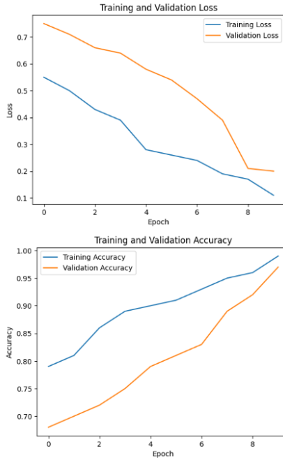
Fig. 11. Training and Validation Loss/ Accuracy for RL-LSTM
