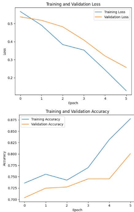
Fig. 3. Training and Validation Loss/ Accuracy for CNN
