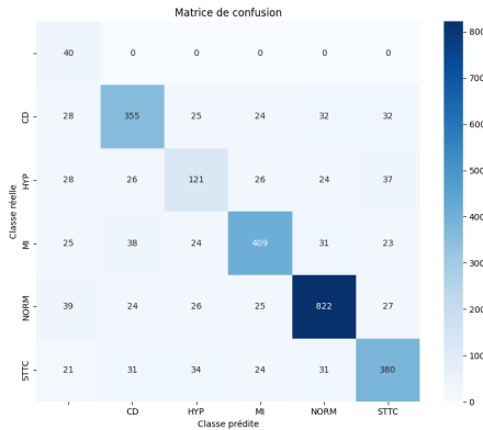
Fig. 4. Confusion Matrix for DNN
