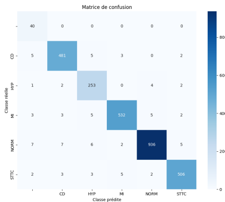
Fig. 10. Confusion Matrix for RL-LSTM
