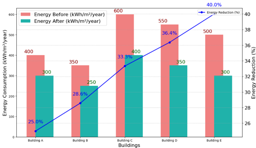
Fig. 1. Energy Consumption Before and After Retrofitting.
