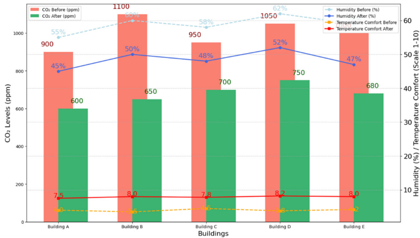
Fig. 2. Indoor Environment Quality Before and After Retrofitting.
