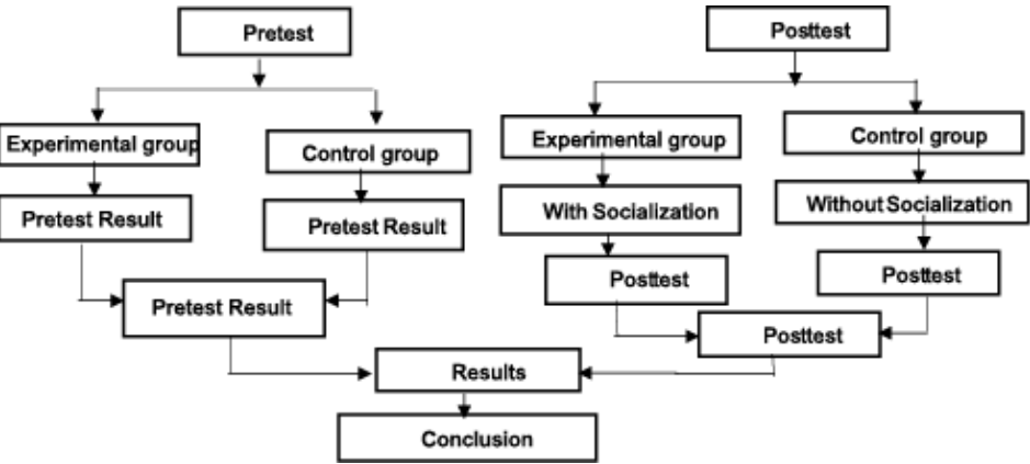
Fig. 1. Implementation Flow
