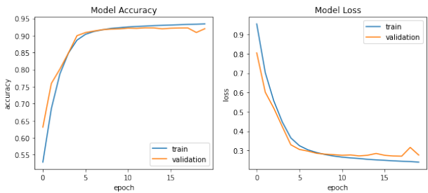
Fig. 4. Model training performance curve
