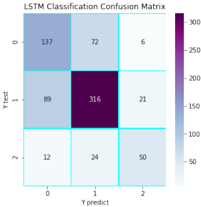
Fig. 5. LSTM Classification Confusion Matrix
