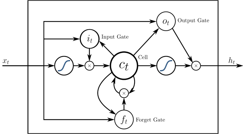
Fig. 3. LSTM structural unit
