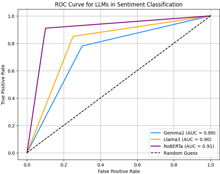
Fig. 4: ROC curves comparison
