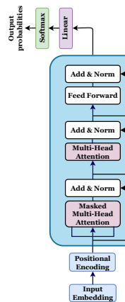
Fig. 2: Decoder-Only Transformer Architectures for LLMs.
