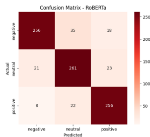
Fig. 7: Confusion matrix illustrating the classification performance of the RoBERTa.
