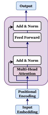
Fig. 3: Encoder-based Transformer Architectures for LLMs.
