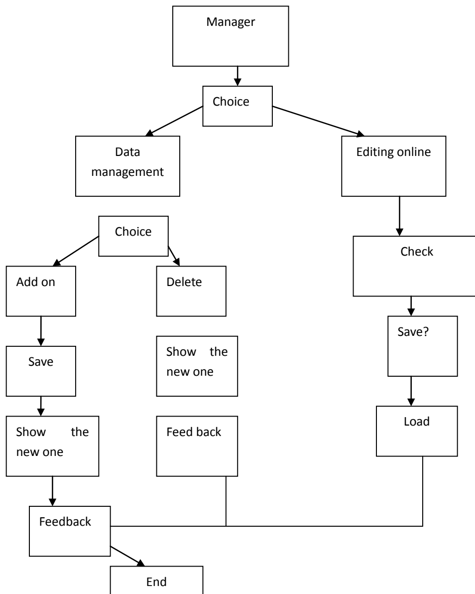
Fig 2. The administrator module flow chart
