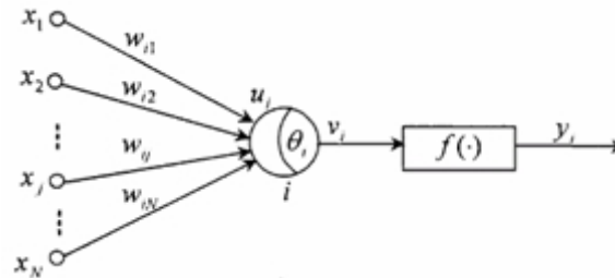
Figure 1. BP Neuron Model
