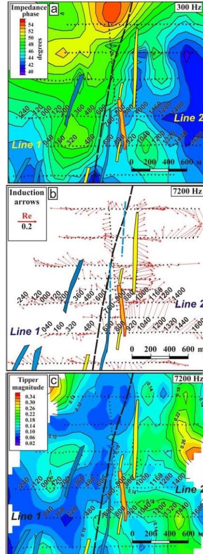
Fig.2 Maps of invariant impedance phase at 300 Hz (a), induction arrows (b) and tipper magnitude (c) at 7200 Hz. Orange veins were found by drilling data till 2013, yellow veins are 2014 boreholes results.
