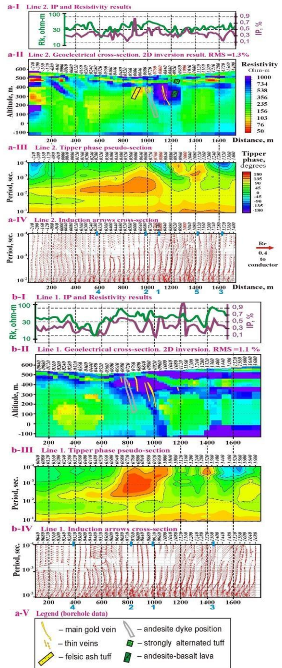
Fig.3 AMP-MVP and IP results comparison along lines 2 (a) and 1 (b). The blue rectangles on the upper part of induction arrows cross-sections (a,b-IV) are resistive zones.
