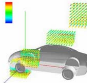
Fig 5. The distribution of electromagnetic field
