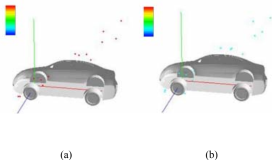
Fig 4. The display of extremum value in electromagnetic field
