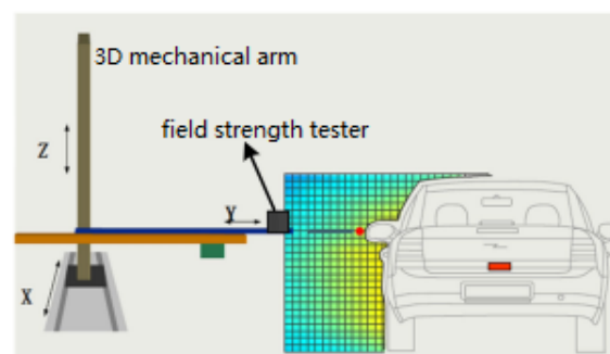
Fig. 1. Mechanical arm automatic moving diagram
