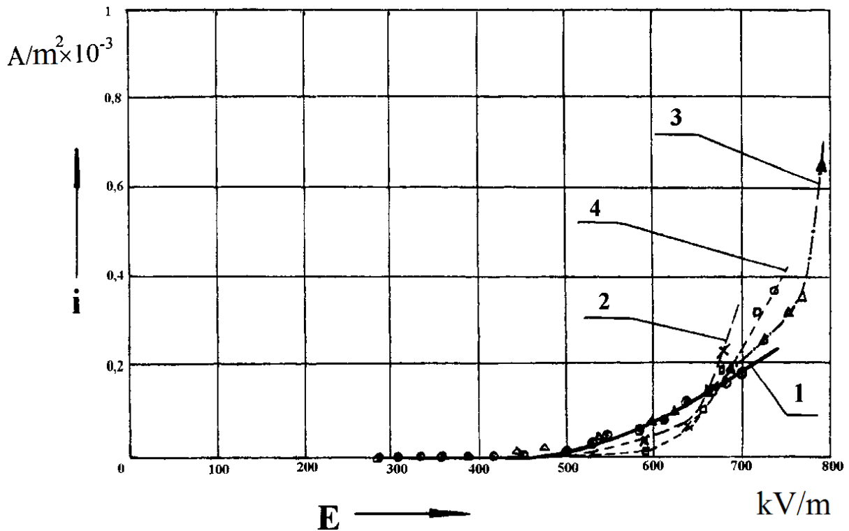
Fig. 2. The volt-amps chamber diagram with pad electrodes: 1- no load operation, (-) on opposed electrode; 2- no load operation, (+) on opposed electrode; 3- barley "Acha" in the gap, (-) on opposed electrode; 4- barley "Acha" in the gap, (+) on opposed electrode.
