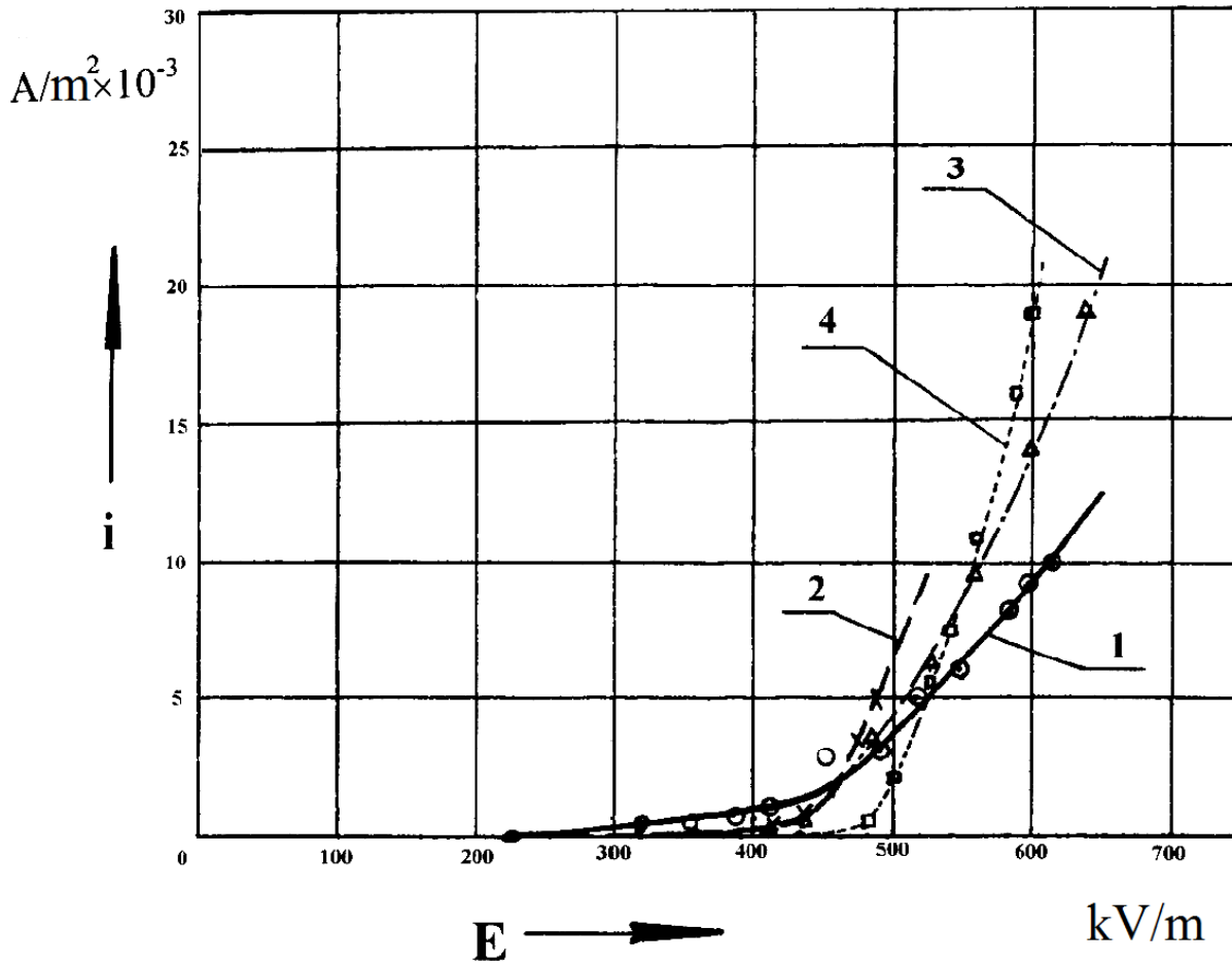
Fig. 1. The volt-amps chamber diagram with needle electrodes: 1- no load operation, (-) on opposed electrode; 2- no load operation, (+) on opposed electrode; 3- barley "Acha" in the gap, (-) on opposed electrode; 4- barley "Acha" in the gap, (+) on opposed electrode.
