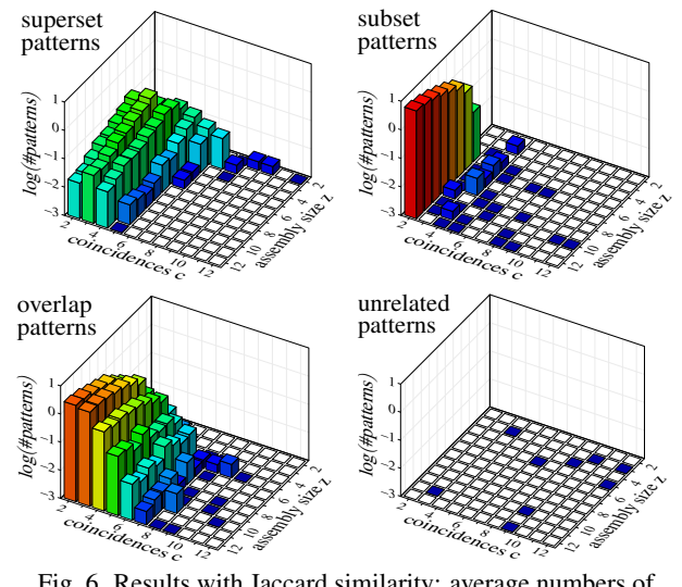
Fig. 6. Results with Jaccard similarity: average numbers of patterns other than the actual (injected) pattern per data set. These patterns may be produced instead of or in addition to the actual (injected) pattern. Especially overlap patterns are usually returned in addition, as can be seen by comparing the diagram with the false negative diagrams in Figure 5. More patterns compared to Figure 4 occur mainly where no detection was possible with influence map overlap support.
