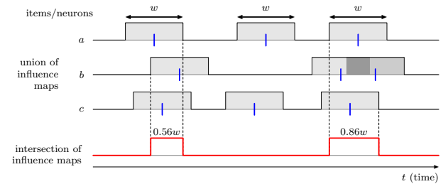
Fig. 1. Support computation for three items a, b, c . Each event has an influence map (represented as a rectangle). If two influence maps overlap, their maximum (union) is computed. (In the diagram, item b has two events, the influence regions of which overlap.) The support results from the integral over the minima of the influence maps (intersections).
