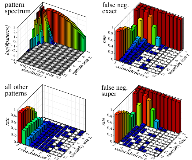
Fig. 5. Results with Jaccard similarity: pattern spectrum and detection performance. Note the lower number of false negatives compared to Figure 3. Trial runs in which patterns other than the actual (injected) pattern are returned are still few and concern mainly patterns with few coincidences, where a superset may be detected. Details about these additional patterns (divided into supersets, subsets, overlap and unrelated patterns) are depicted in Figure 6.
