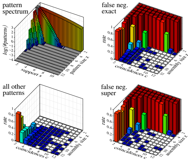
Fig. 3. Experimental results with influence map overlap support: pattern spectrum and detection performance. Trial runs in which patterns other than the actual (injected) pattern are returned are few and concern mainly patterns with few coincidences, where a superset may be detected. Details about these additional patterns (divided into supersets, subsets, overlap and unrelated patterns) are depicted in Figure 4.
