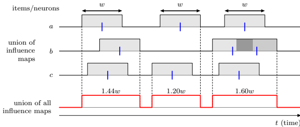
Fig. 2. Additional computations for the Jaccard index for three items a, b, c (cf. Figure 1). The extent results from the integral over the maxima of the influence maps (union). The resulting Jaccard index is J(\{a, b, c\}) = \frac{0.56w + 0.86w}{1.44w + 1.20w + 1.60w} = \frac{1.42}{4.24} \approx 0.335 .
