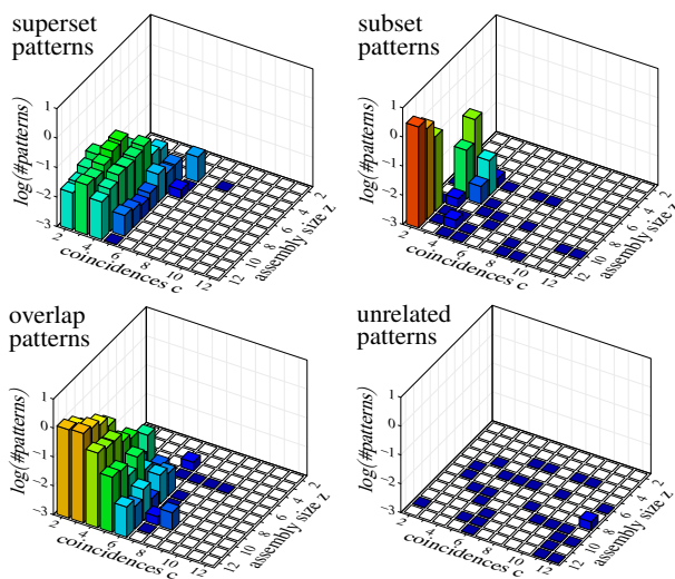
Fig. 4. Experimental results with influence map overlap support: average numbers of patterns other than the actual (injected) pattern per data set. These patterns may be produced instead of or in addition to the actual (injected) pattern. Especially overlap patterns are usually returned in addition, as can be seen by comparing the diagram with the false negative diagrams in Figure 3.
