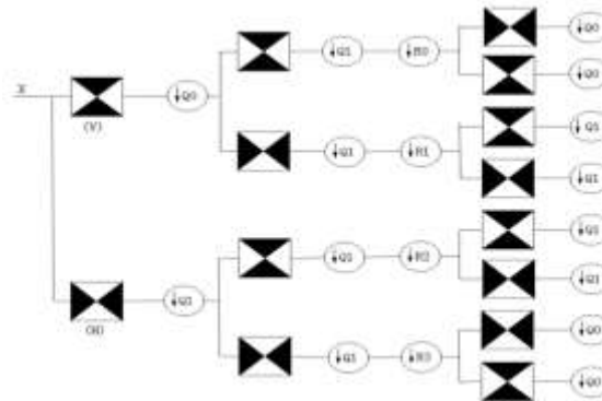
Figure3. Subband division of direction filter
