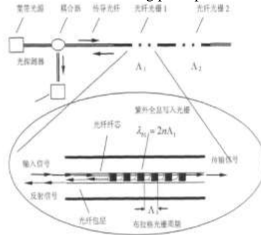
Figure 1. Working Principle of Fiber Grating Sensing
