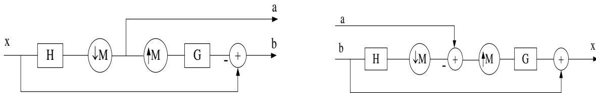
(a) Decomposition of fiber Bragg grating signals (b) Reconstruction of fiber Bragg grating signals
