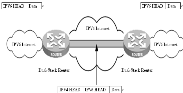
Figure 2 The IPv6 passing through IPv4 Tunnel
