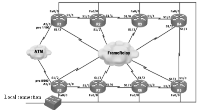
Figure 3 6to4 tunnel topology diagram
