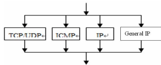
Figure 2. Rules optimization design
