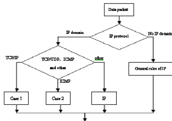
Figure 3. General structure of rule set optimization
