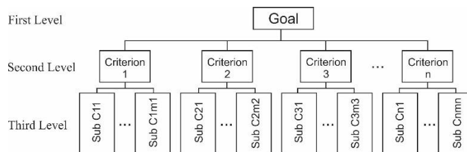
Fig. 1. Hierarchical structure of the AHP
