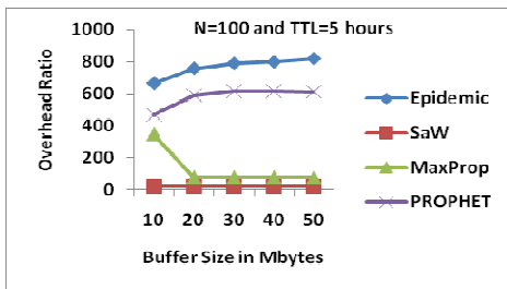
Fig.4.Impact of varying buffer size on overhead ratio
