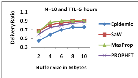
Fig.1. Impact of varying buffer size on delivery ratio
