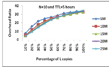
Fig. 9. Impact of varying L copies on overhead ratio
