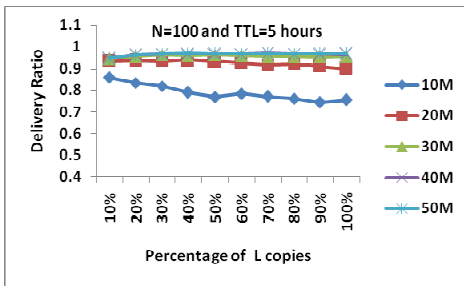
Fig.8. Impact of varying L copies on delivery ratio
