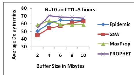
Fig.5. Impact of varying buffer size on average delay
