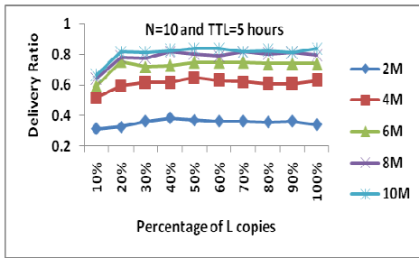
Fig. 7. Impact of varying L copies on delivery ratio
