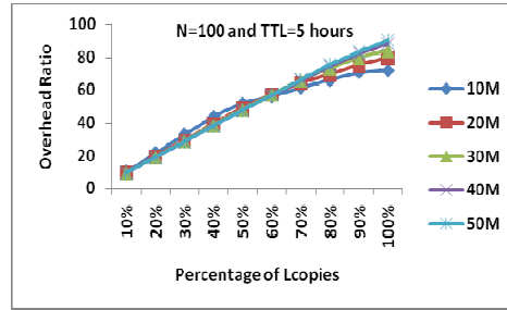
Fig.10. Impact of varying L copies on overhead ratio
