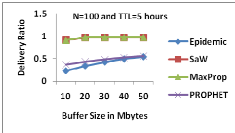
Fig. 2. Impact of varying buffer size on delivery ratio
