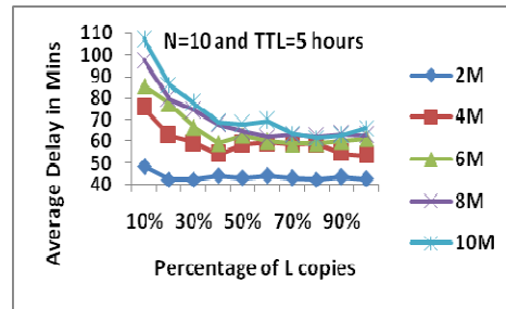
Fig.11. Impact of varying L copies on average delay
