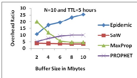
Fig. 3. Impact of varying buffer size on overhead ratio
