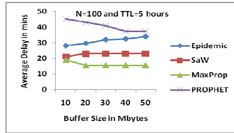
Fig.6. Impact of varying buffer size on average delay
