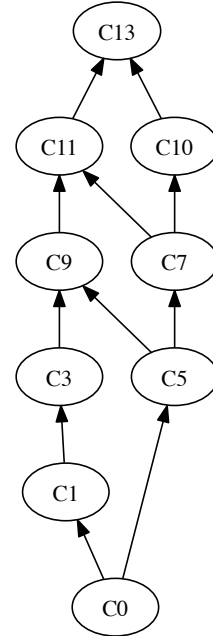
Figure 4: Concept lattice (\mathcal{M}_{0.8}, \preceq)
