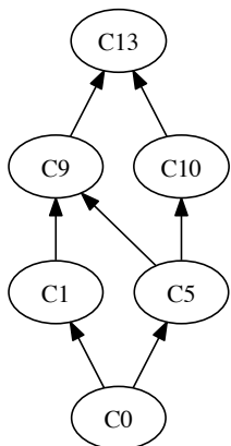
Figure 5: Concept lattice (\mathcal{M}_{1,0}, \preceq)
