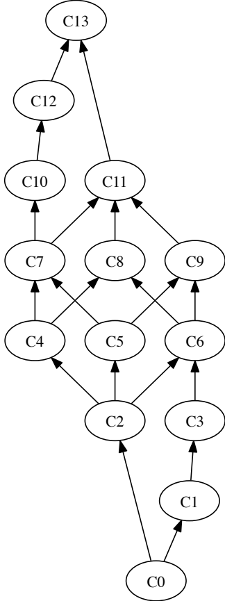
Figure 3: The Hasse diagram of (\mathcal{M}, \preceq)
